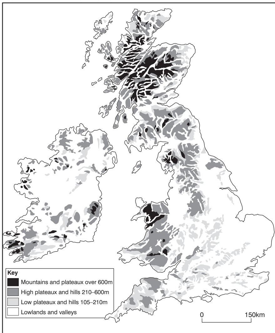
Figure 1: Distribution of relief regions
